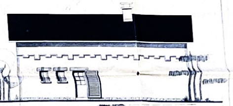
FACADE NORD.
