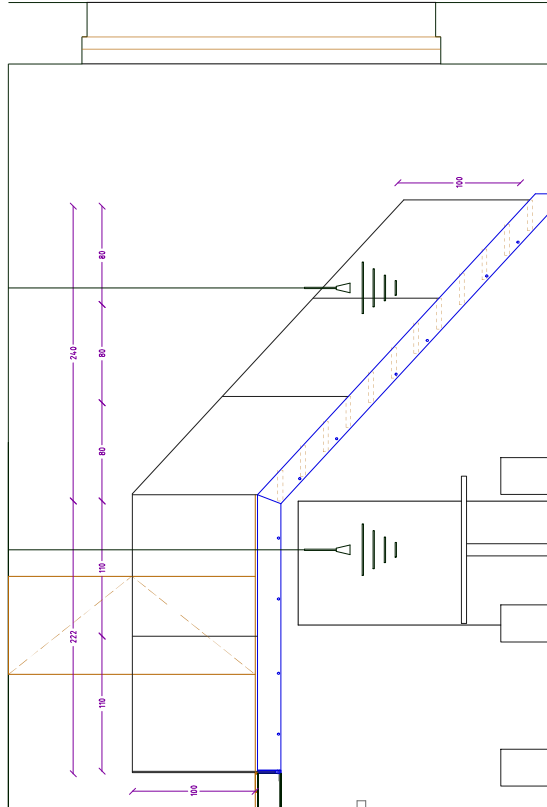
LEFT ELEVATION 1/20
