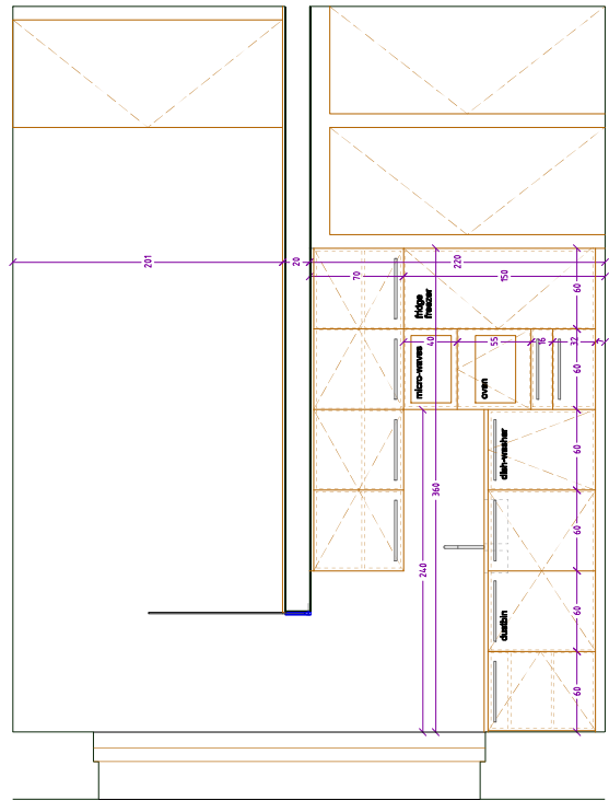
LEFT ELEVATION
