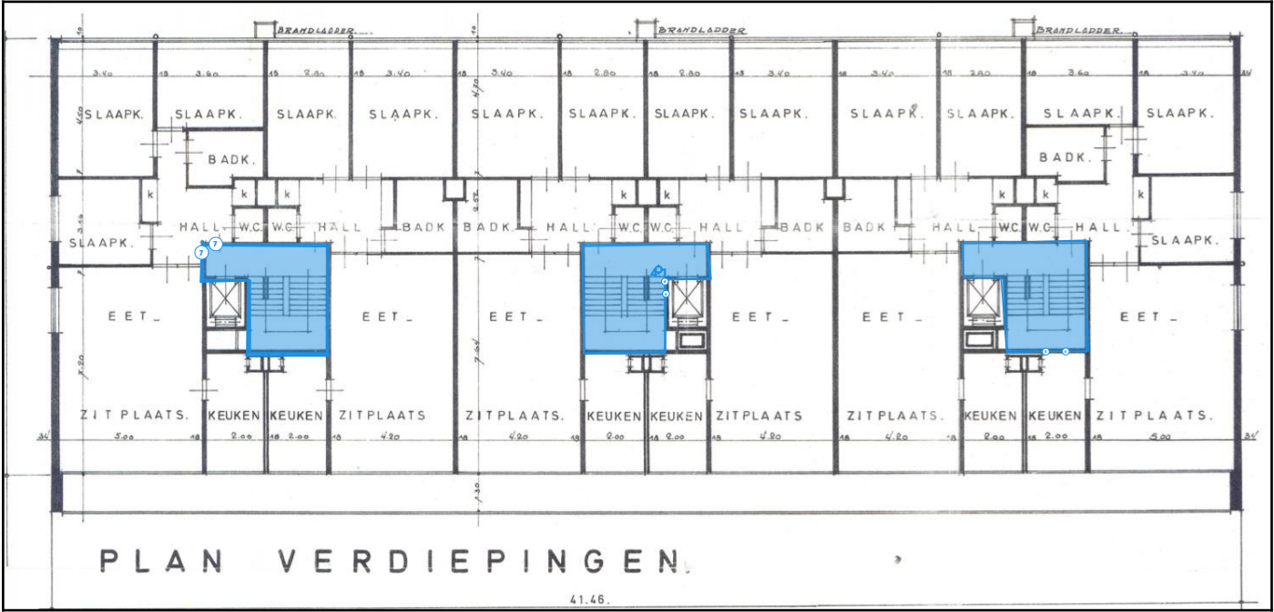
Legende van plan 1.3: Verdieping +1
