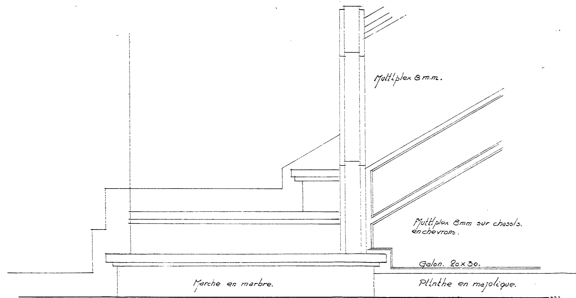
DETAILS ESCALIERS. 70%
