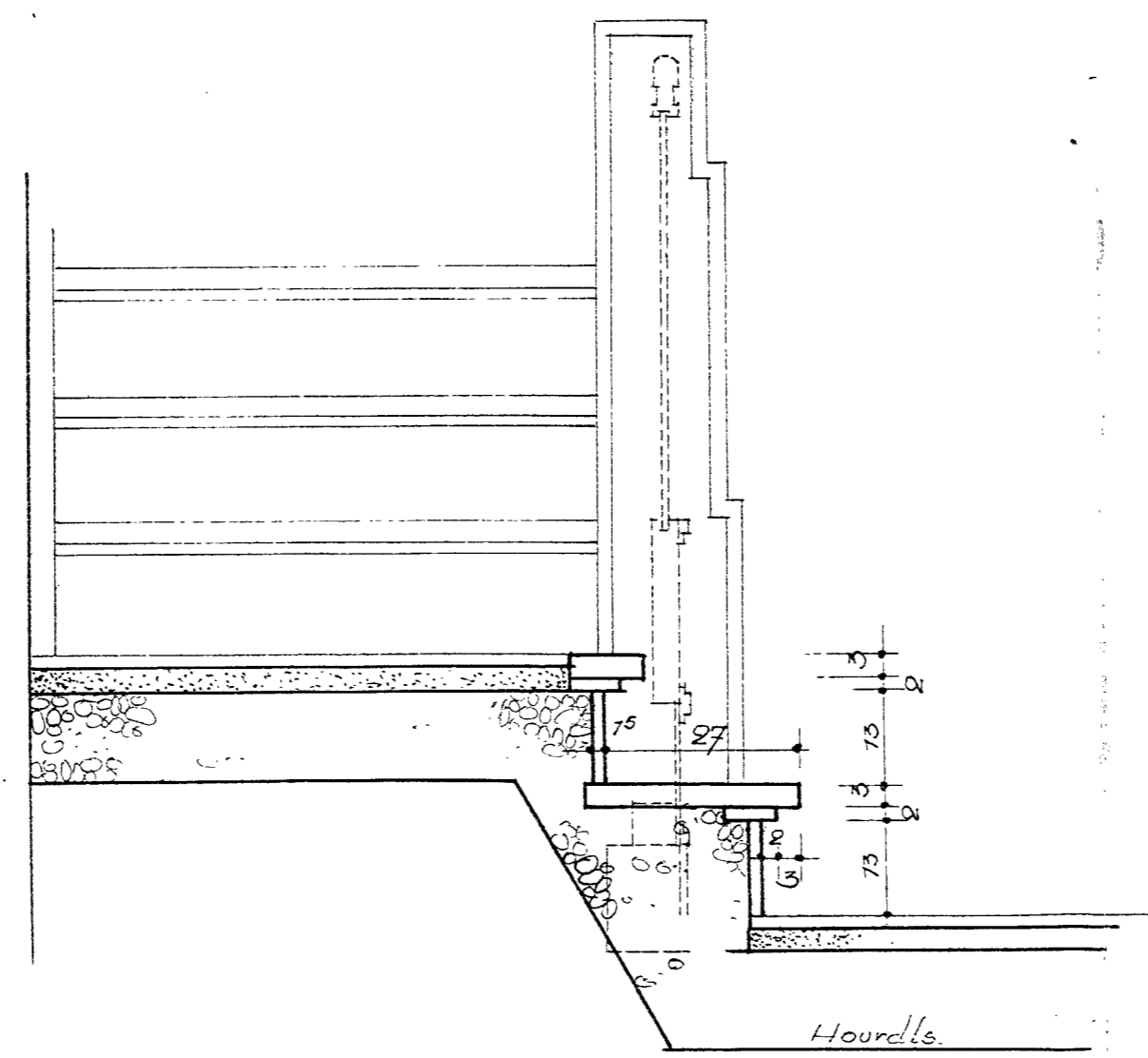
DETAILS ESCALIERS. 70%
